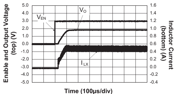
Soft Start ( V_{IN} = 3.6V ; V_{OUT} = 1.8V ; 500mA)
