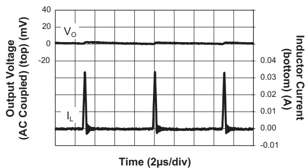
Output Ripple
