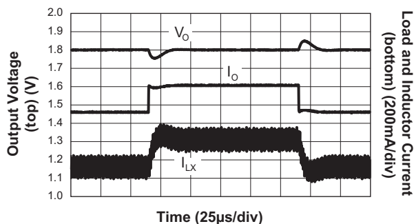
Load Transient Response (350mA to 500mA; V_{IN} = 3.6V ; V_{OUT} = 1.8V ; C_{OUT} = 4.7\mu F ; C_{FF} = 100pF )
