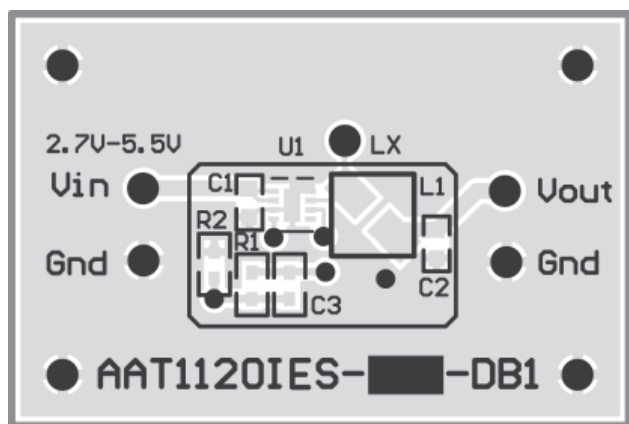
Figure 2: AAT1120 Evaluation Board Top Side Layout.
