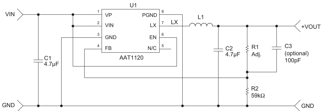
Figure 1: AAT1120 Schematic.
