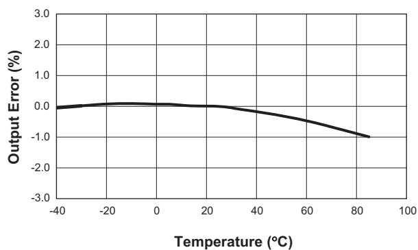
Output Voltage Error vs. Temperature ( V_{IN} = 3.6V ; V_{OUT} = 1.8V ; I_{OUT} = 500mA )
